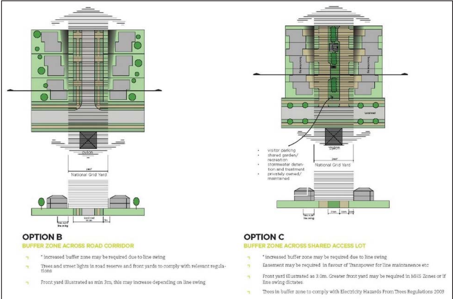
Figure 13. Possible design options for subdivision layouts within the National Grid Subdivision Corridor - Option B and C
